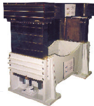
Corrosion-resistant elevating table for tests in a climatic and corrosion chamber: Therefore the table top is made from aluminium/bronze.
