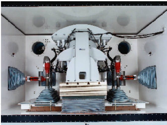
Elevating table (with standard axle fixture mounted on top) in a climatic chamber
